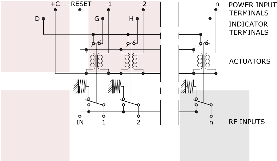
SCHEMATIC DIAGRAM
