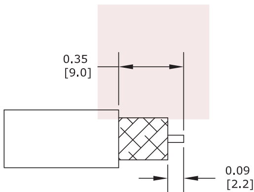
STRIPPING DIMENSIONS
