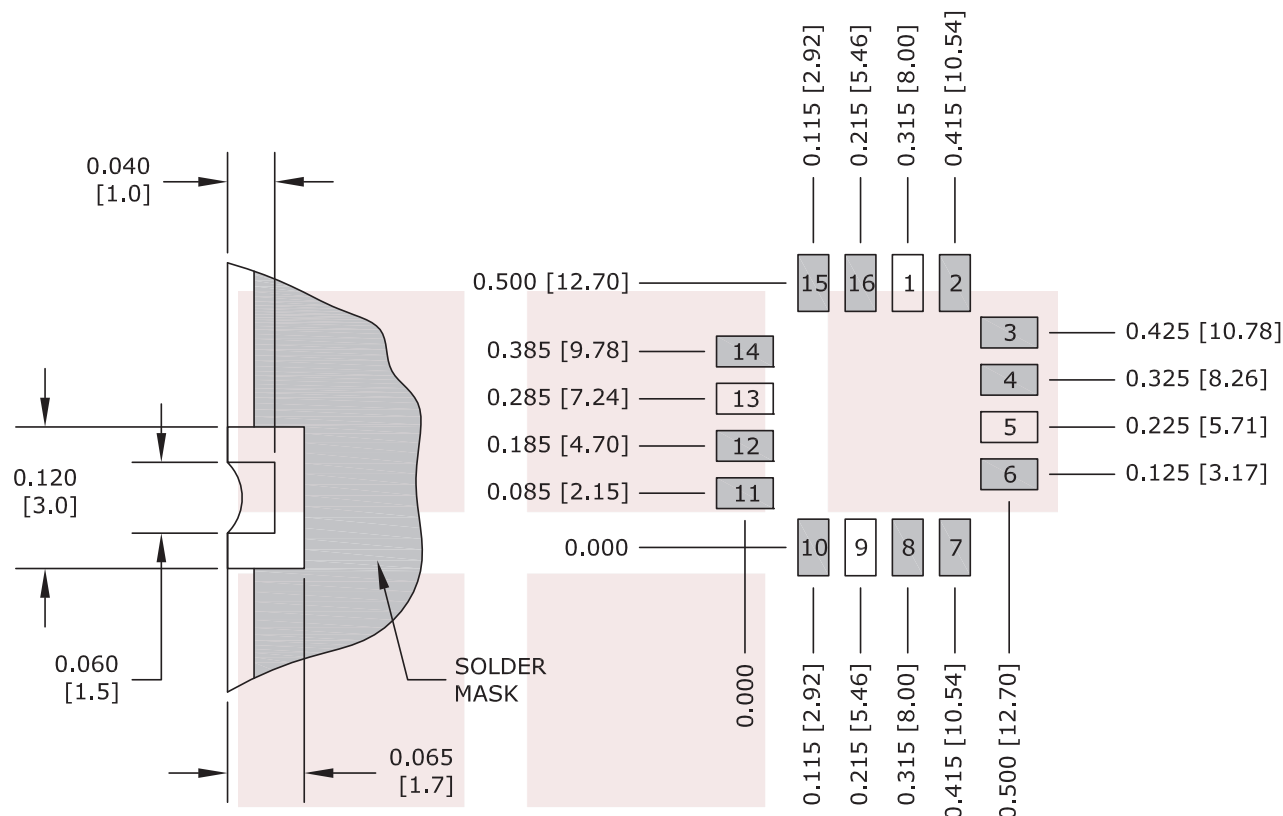
PAD DETAIL
