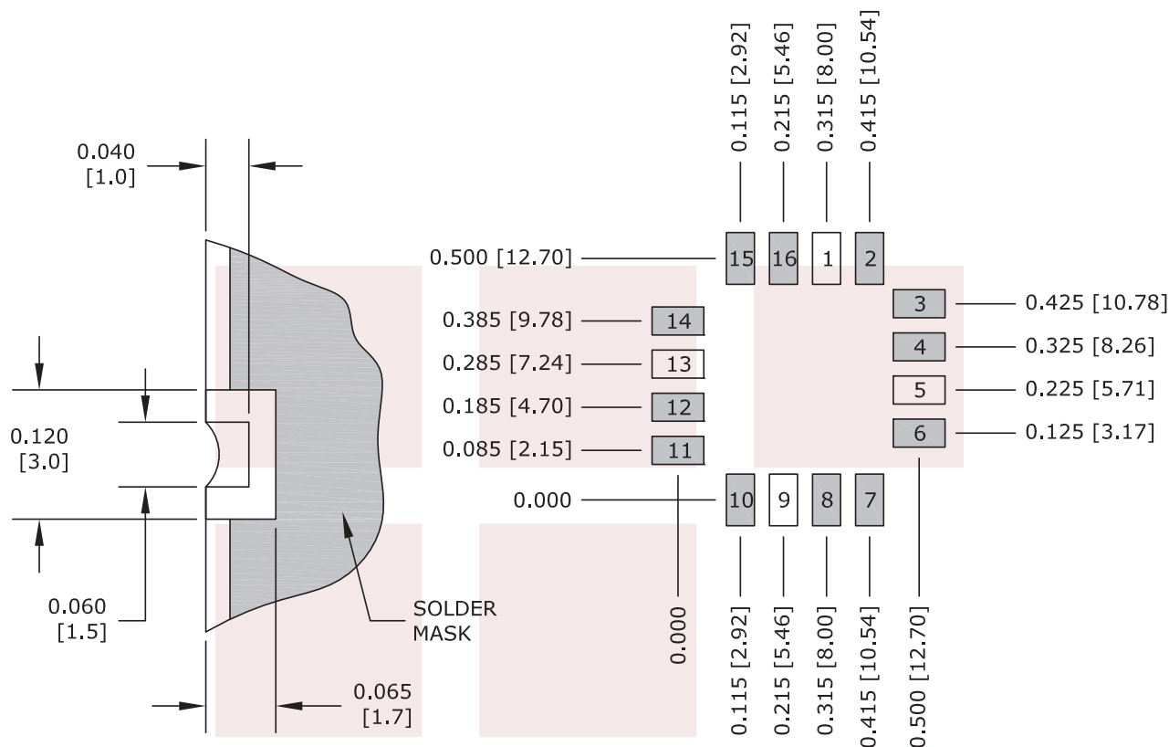
PAD DETAIL
