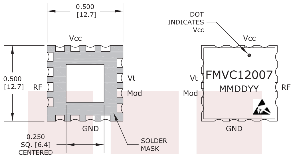
BOTTOM VIEW
