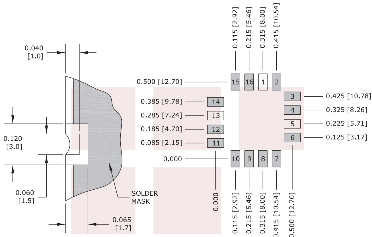
PAD DETAIL
