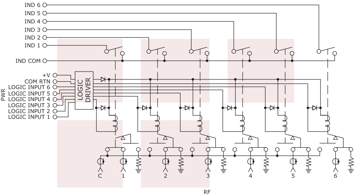
SCHEMATIC LATCHING SELF CUT-OFF SHOWN IN POSITION 1
