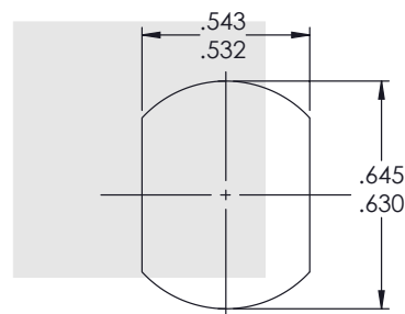
MOUNTING HOLE
