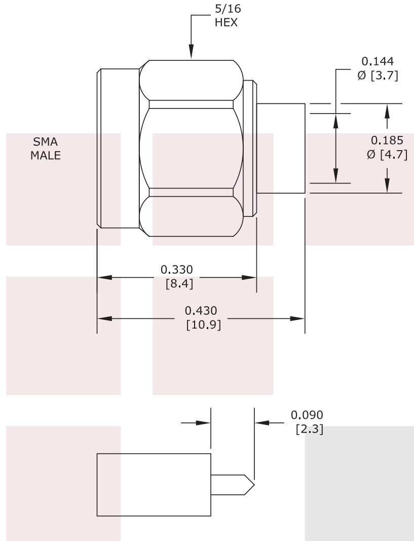
STRIPPING DIMENSIONS
