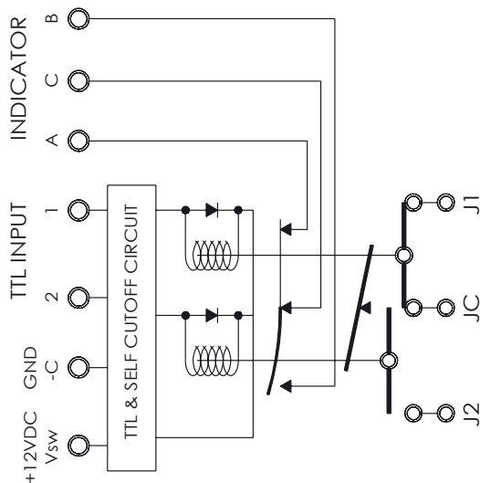
SCHEMATIC
