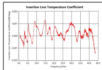
Insertion Loss Temperature Coefficient
