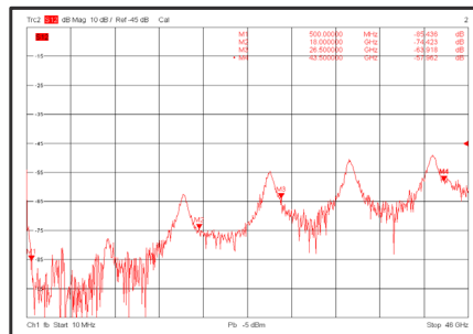
Isolation @+25°C
