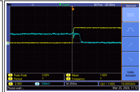
Switching Speed
