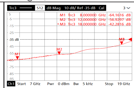
Isolation @+85°C
