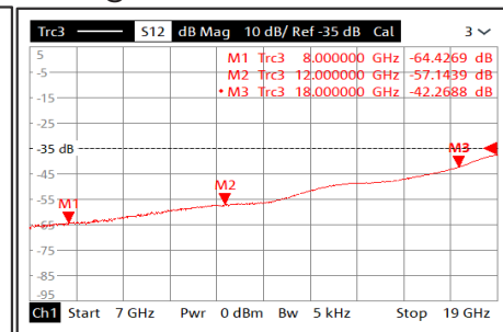
Isolation @-40°C
