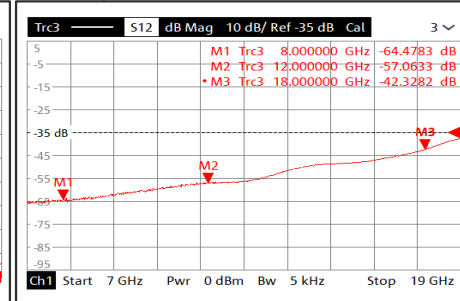
Isolation @+25°C
