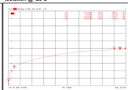
Isolation @+25°C
