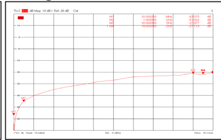
Isolation @+85°C
