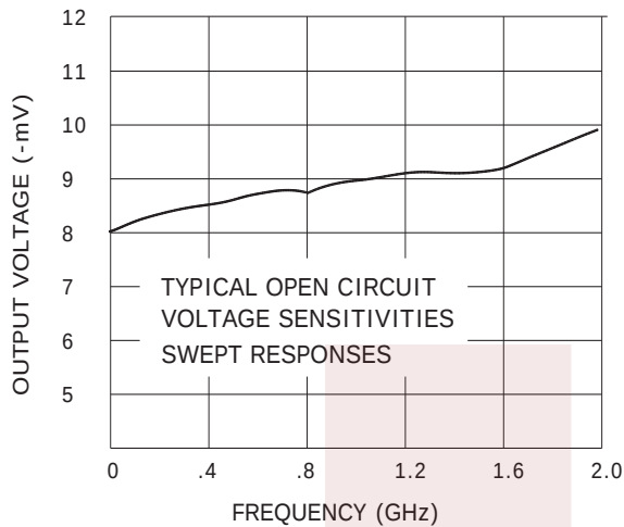
Typical Performance at +25° C
