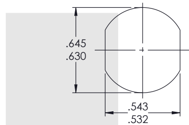
MOUNTING HOLE
