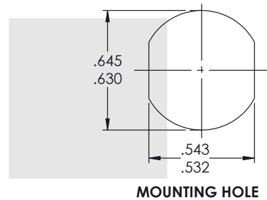
MOUNTING HOLE
