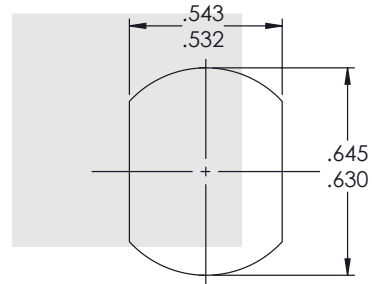
MOUNTING HOLE
