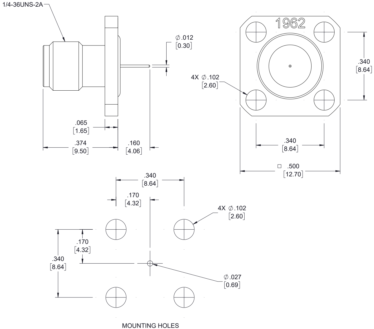
MOUNTING HOLES
