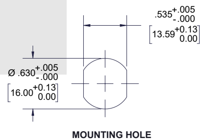
MOUNTING HOLE
