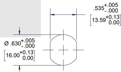
MOUNTING HOLE
