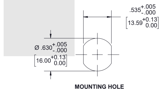
MOUNTING HOLE
