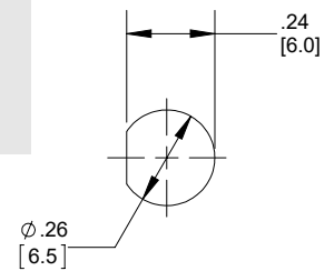
MOUNTING HOLE
