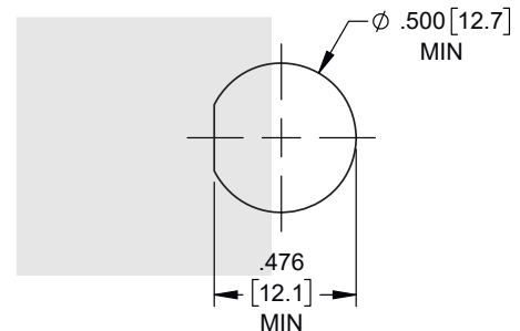
MOUNTING HOLE
