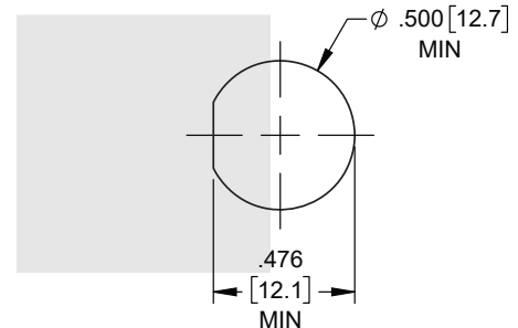
MOUNTING HOLE
