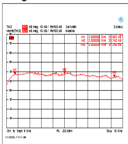
Gain @+25°C
