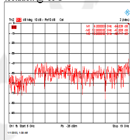
Isolation @+85°C
