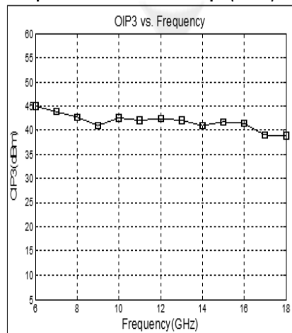
Output Third Order Intercept (OIP3)
