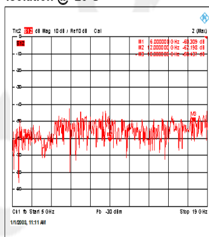
Isolation @+25°C
