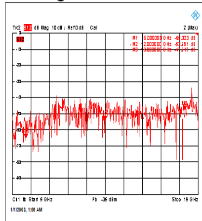
Isolation @-40°C
