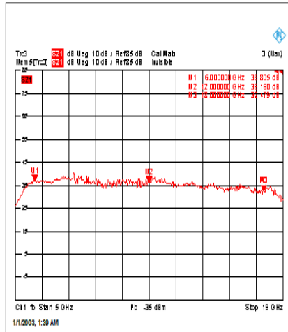
Gain @+85°C
