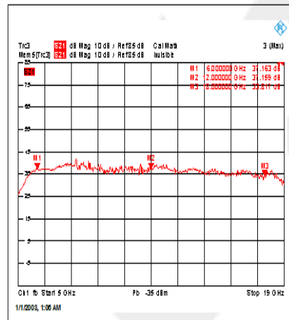
Gain @-40°C
