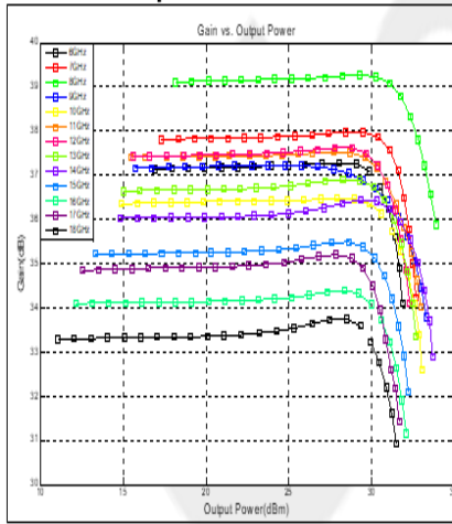
Gain vs. Output Power
