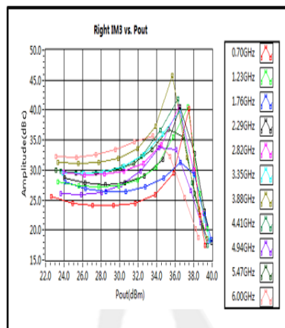
Right IM3 vs. Pout
