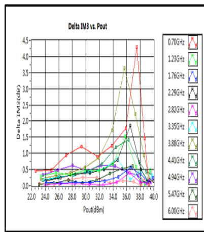
Delta IM3 vs. Pout
