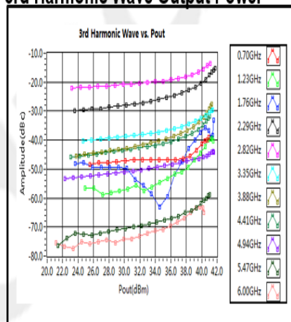
3rd Harmonic Wave Output Power
