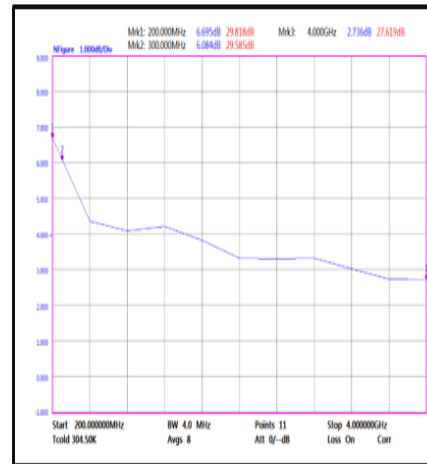
Noise Figure(0.2GHz-4GHz)
