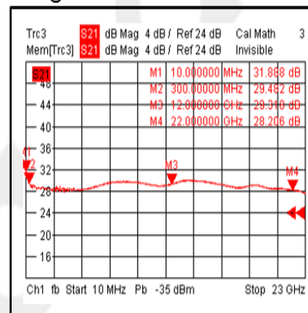
Gain@-40°C
