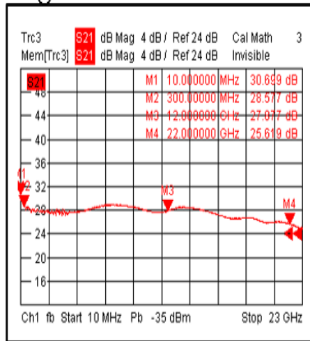
Gain@+25°C
