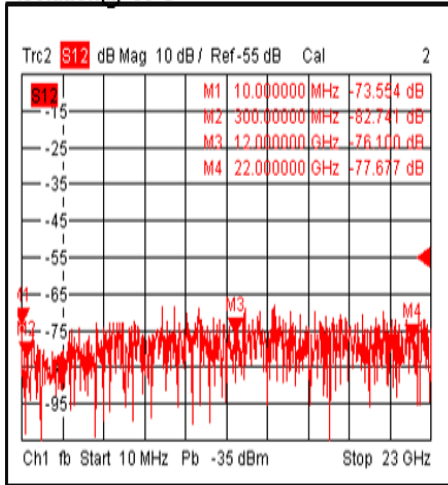
Isolation@+85°C
