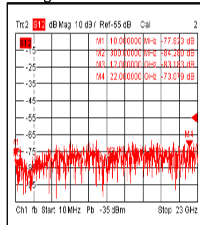
Isolation@-40°C
