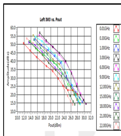
Left IM3 vs. Pout
