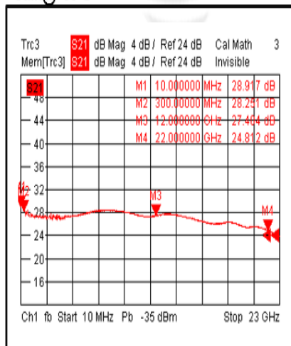
Gain@+85°C
