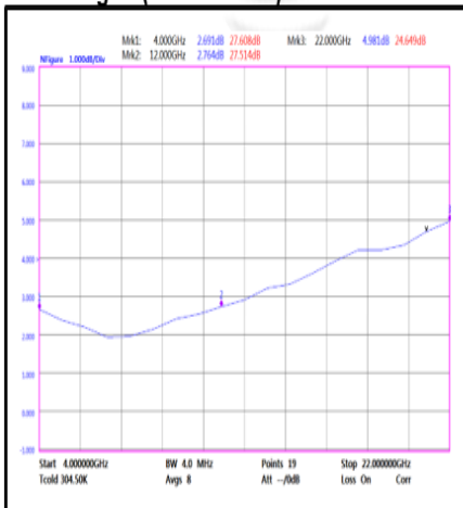
Noise Figure(4GHz-22GHz)
