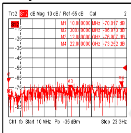
Isolation@+25°C
