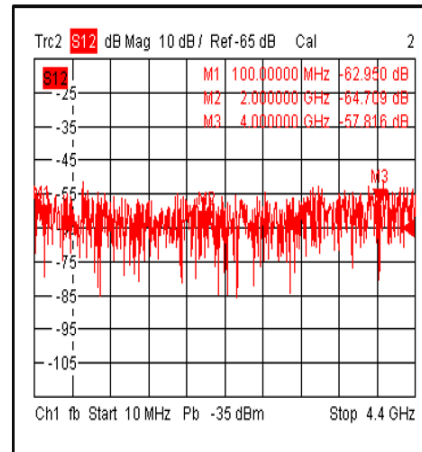
Isolation@-40°C
