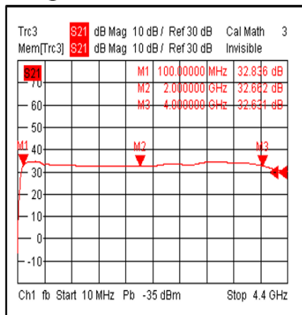
Gain@+85°C
