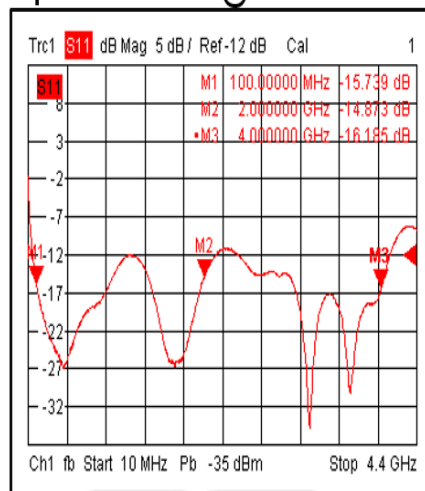
Input Return Loss@+25°C
