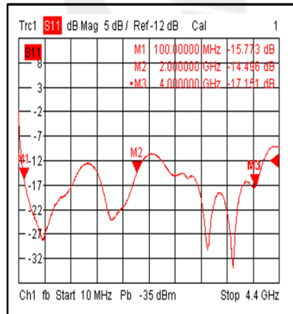
Input Return Loss@-40°C
