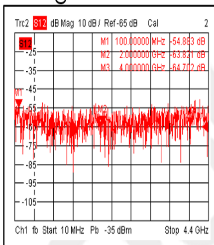
Isolation@+25°C
