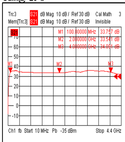
Gain@+25°C
