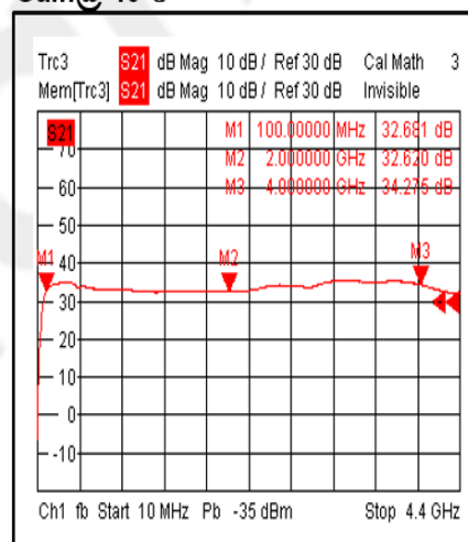
Gain@-40°C
