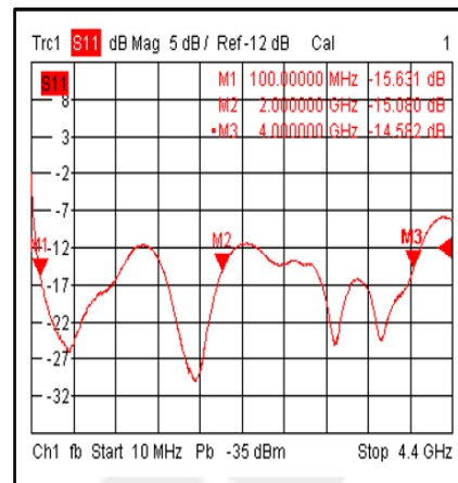
Input Return Loss@+85°C
