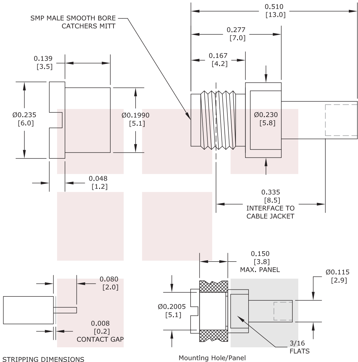
STRIPPING DIMENSIONS
