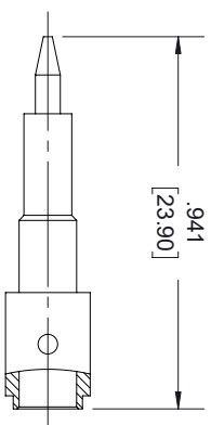
CONTACT
