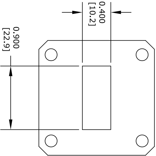
UG 39/U WR 90 COVER FLANGE
