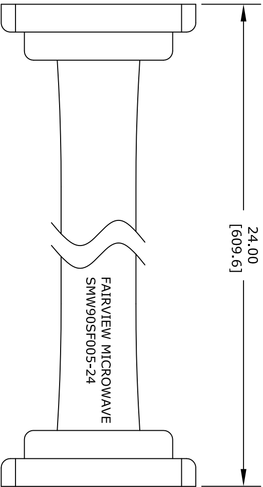
UG 39/U WR 90 COVER FLANGE
