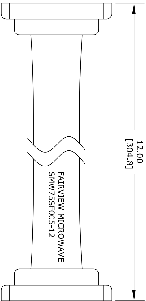
WR 75 COVER FLANGE
