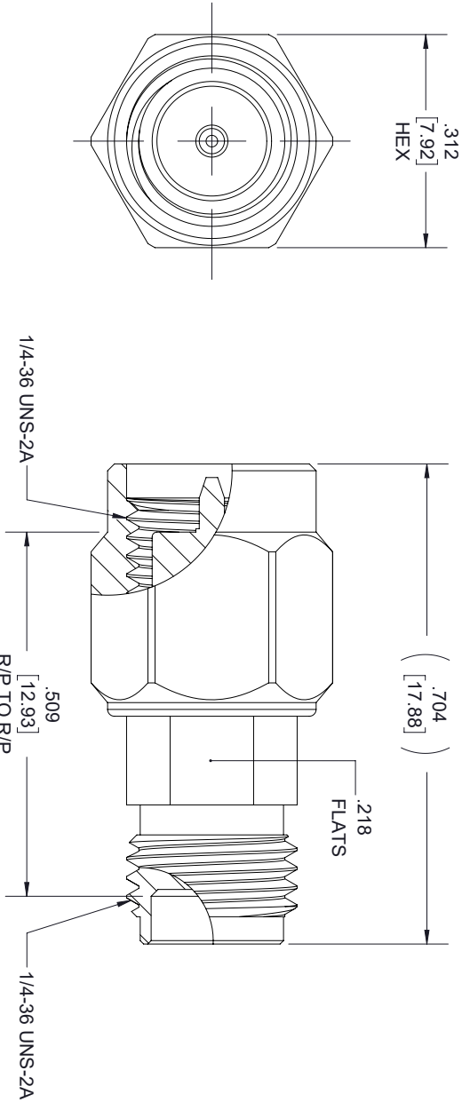
SMA MALE
