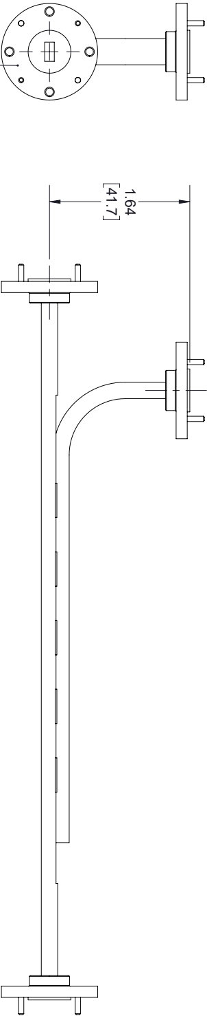
WR-22 WAVEGUIDE UG-383/U ROUND COVER FLANGE TYP
