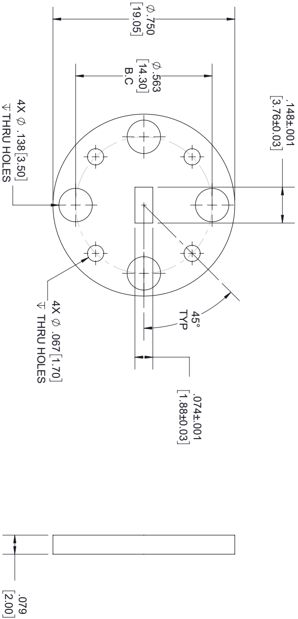
WR-15 WAVEGUIDE UG-385/U ROUND COVER FLANGE
