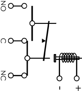
SCHEMATIC SHOWN IN FAILSAFE POSITION
