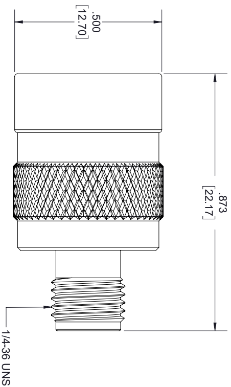
3.5mm FEMALE SHORT
