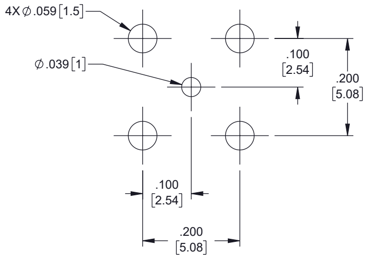
RECOMMENDED PANEL CUTOUT PATTERN
