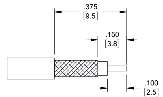
STRIPPING DIMENSIONS
