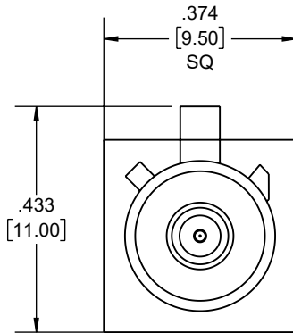
FAKRA PLUG B CODING WHITE
