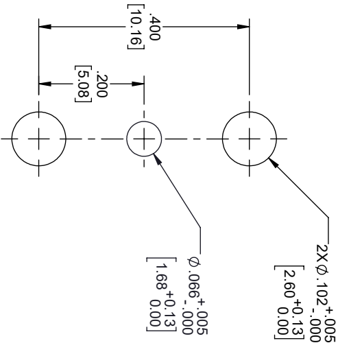
MOUNTING HOLES PATTERN
