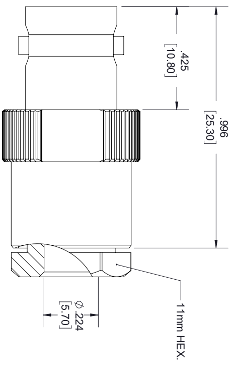
50 Ohm BNC FEMALE
