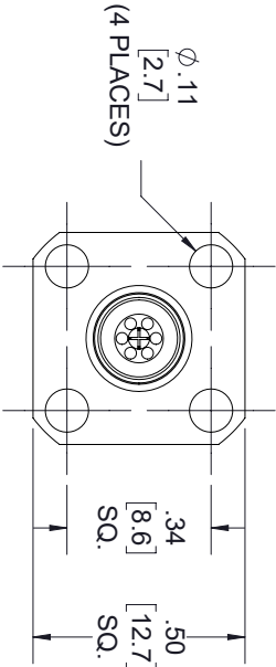
MOUNTING HOLES
