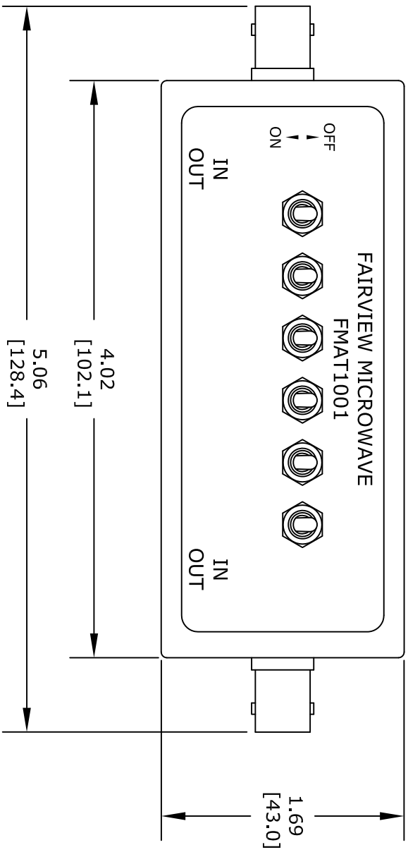
TOP VIEW
