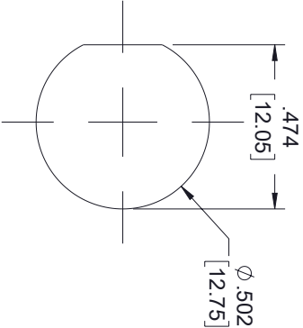
MOUNTING HOLE
