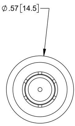
TNC MALE
