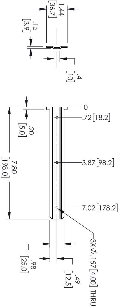
SLIDE BRACKET
