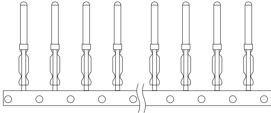
STANDARD MALE CONTACTS, 24-28 AWG
