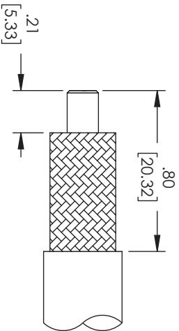
RECOMMENDED CABLE STRIPPING DIMENSIONS
